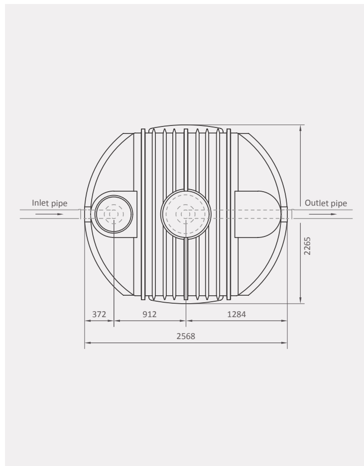
Top view
