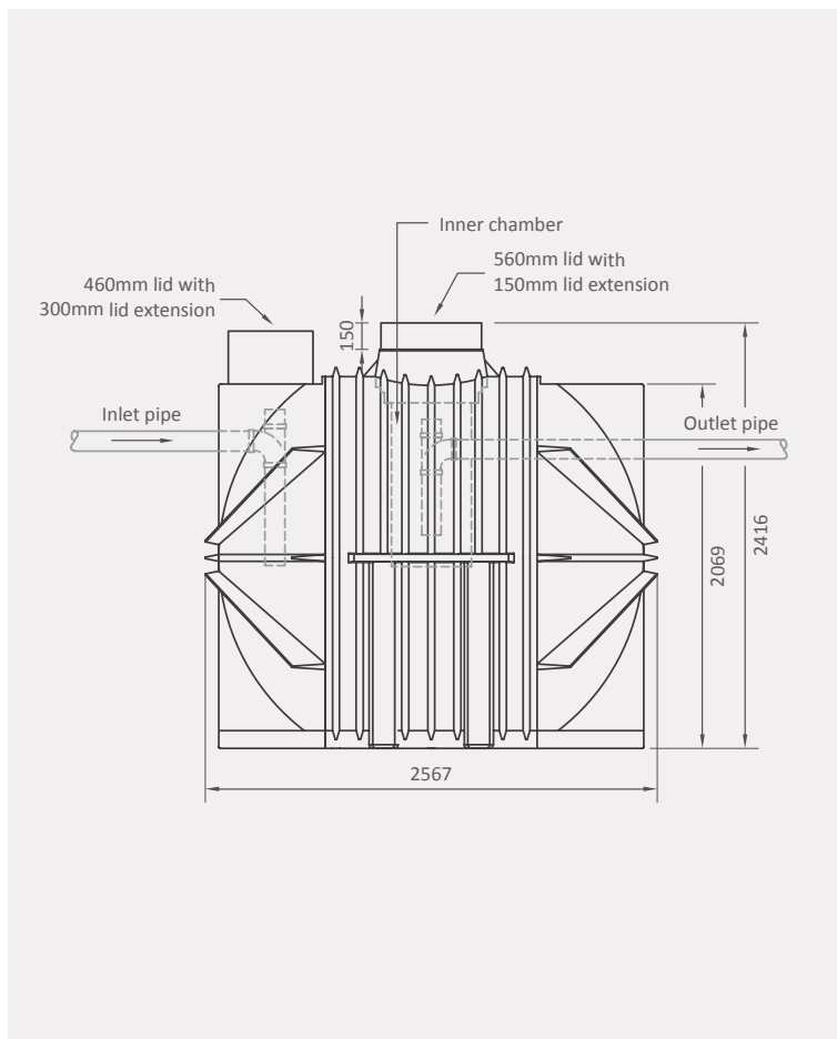
Side view
