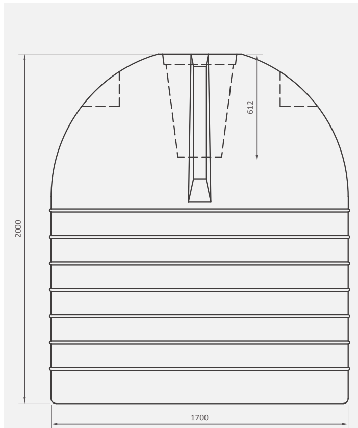
Side view
