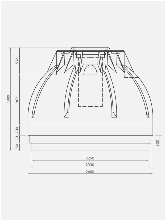
Side view
